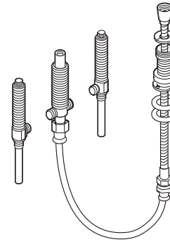
Roman Tub With Built-In Diverter Rough-In Valve (Adjustable Type)
