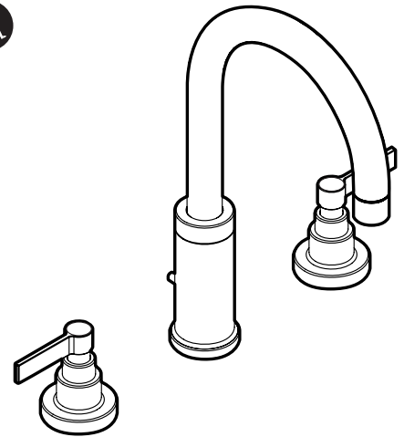
Solace™ Two-Handle Widespread Lavatory Faucet Models: S478, S478BN
